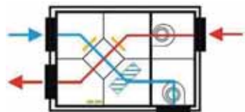
MODELES CADB/CADT-DC 05 / 08 / 18 / 30 / 45 / 56 EH DP
